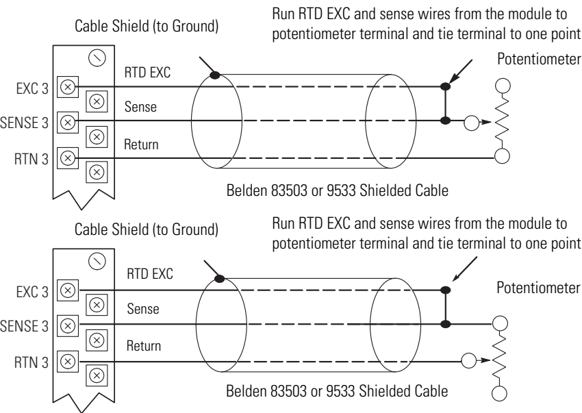
Three Wire Potentiometer Configuration
