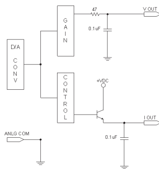
Simplified Output Circuit Diagram
