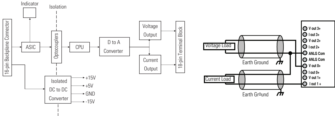
Simplified Schematic
