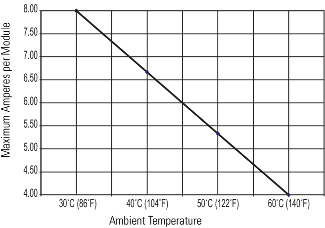
1769-OB16P Maximum Amperes per Module vs. Temperature
