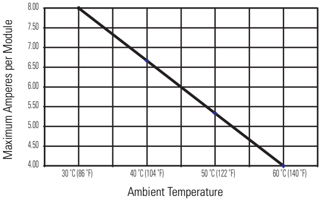
1769-OV16 Maximum Amperes per Module versus Temperature
