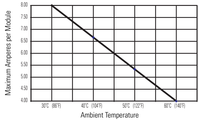
1769-OB16 Maximum Amperes per Module vs. Temperature
