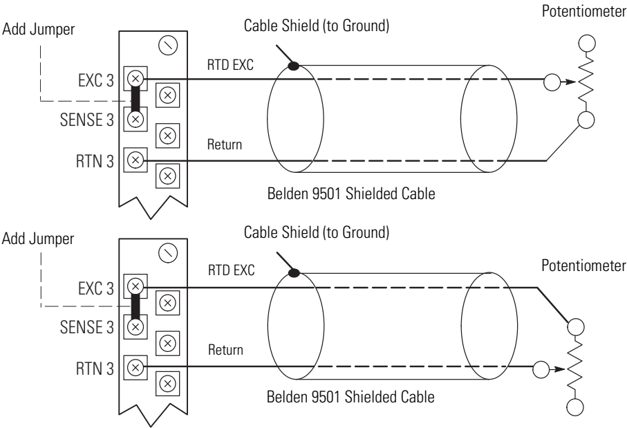
Two Wire Potentiometer Configuration
