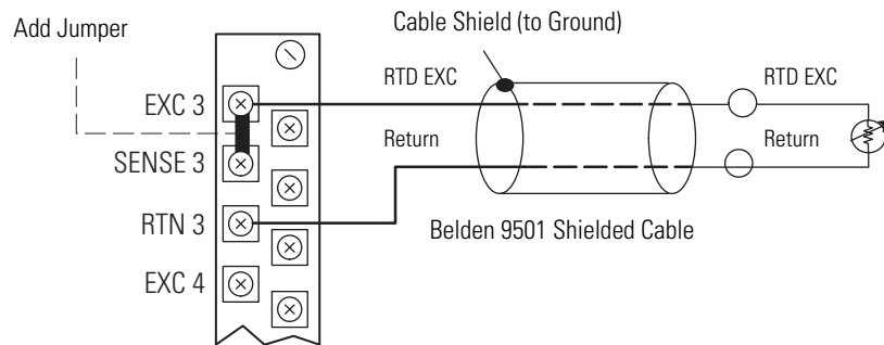
Two Wire RTD Configuration
