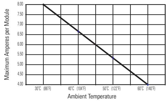
1769-OB32 Maximum Amperes per Module vs. Temperature
