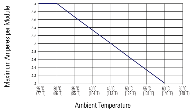
1769-B00LEAN Maximum Amperes per Module versus Temperature
