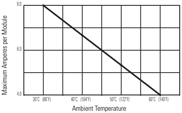
1769-0A16 Maximum Amperes per Module vs. Temperature
