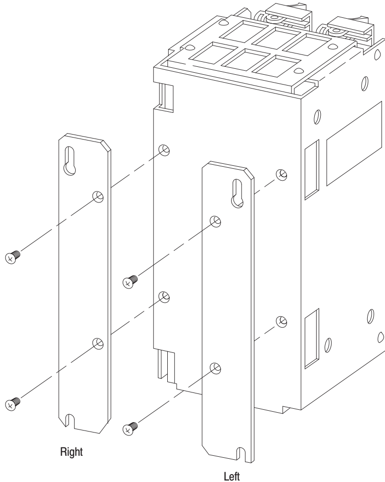
Figure 2 1771-PSC Mounting Flanges Removal/Installation
