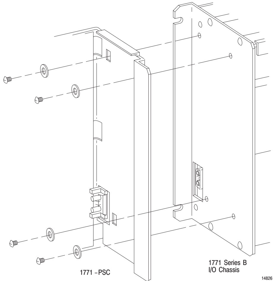
Figure 3 Connector Adjustment Locations
