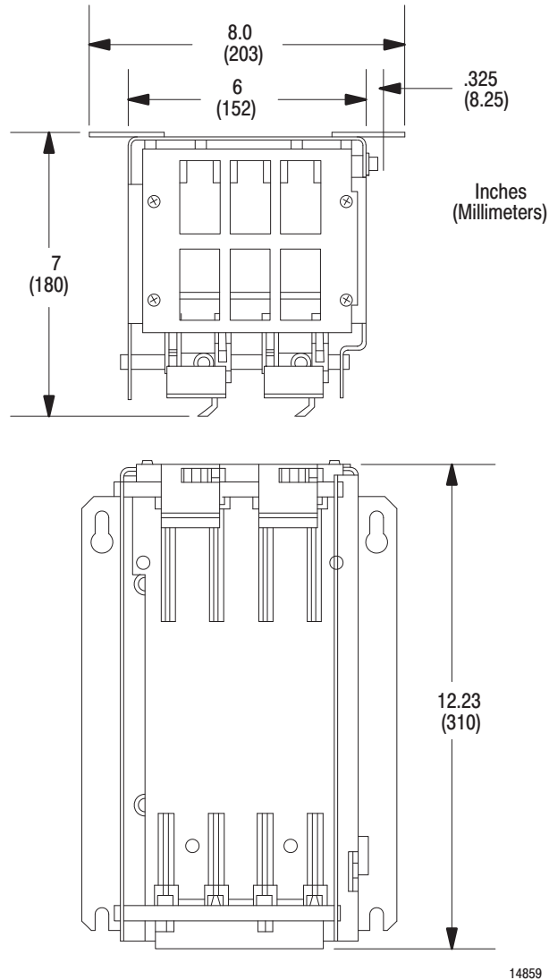
Figure 1 Power Supply Chassis Dimensions
