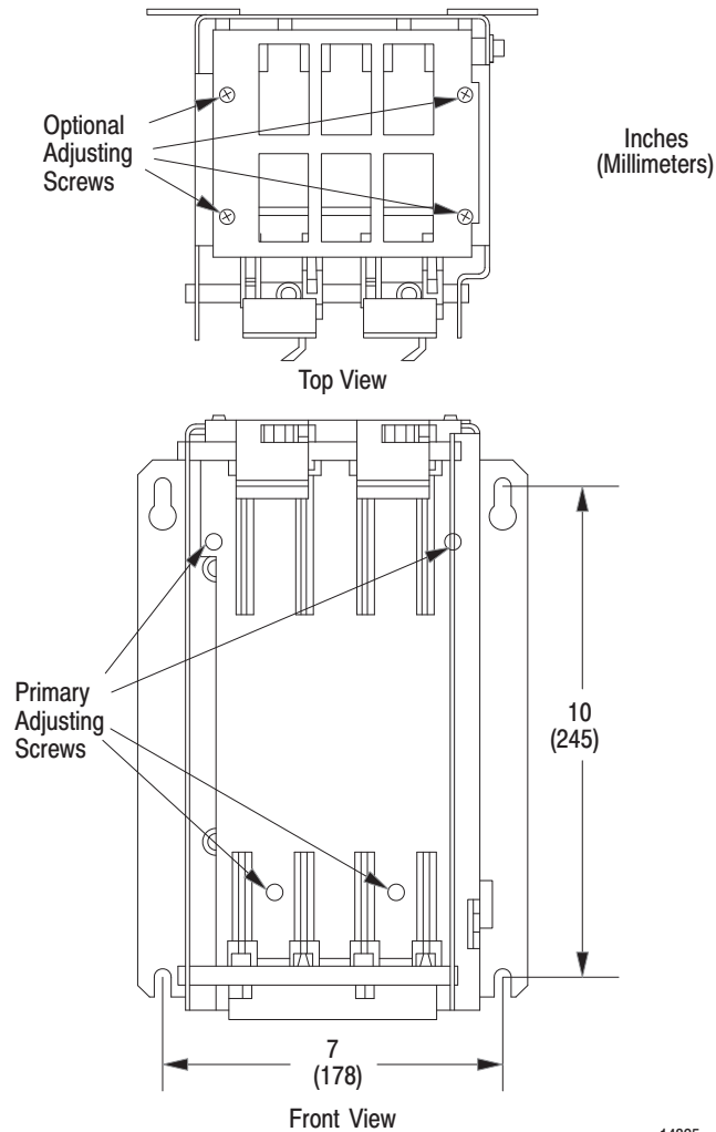
Figure 4 Mounting the 1771-PSC to a 1771 Universal I/O Chassis
