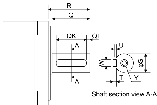
Variable dimension table [Unit: mm]
