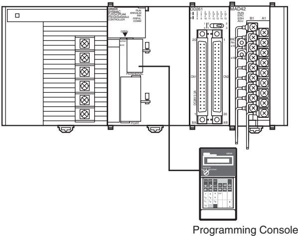
Programming Console
