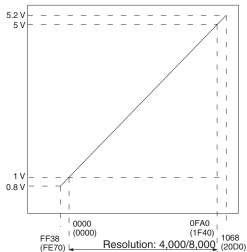
Analog output signal
