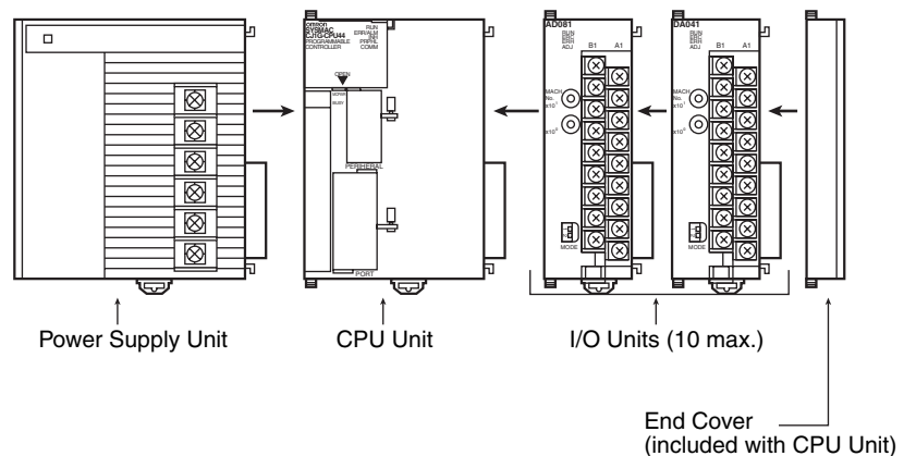
CPU Rack
