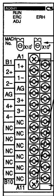
With Terminal Block
