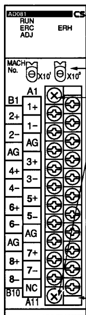
With Terminal Block
