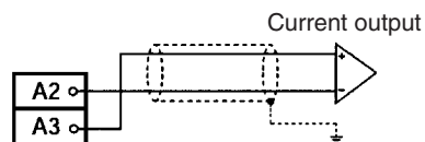
CS1W-DA041 (current output)
