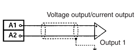
CS1W-DA08V/08C CS1W-DA041 (voltage output)
