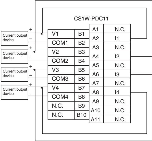
Current inputs
