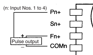
Sensor Power Supply (Connected to 3-wire Sensor)
