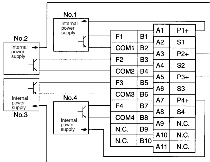
CS1W-PPS01 Isolated-type Pulse Input Unit
