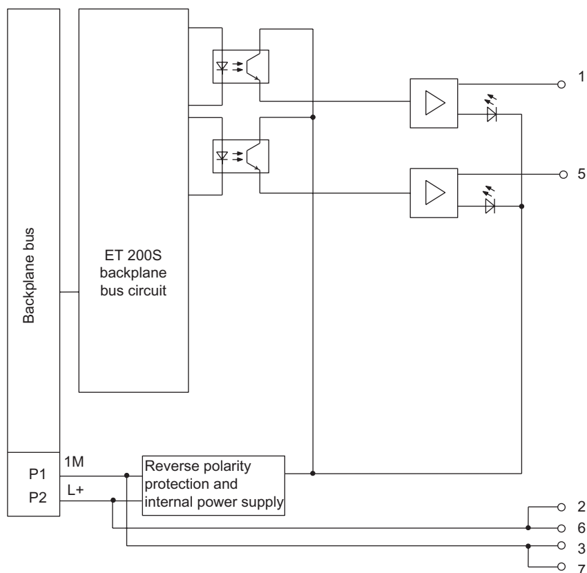
Figure 1-1 Block diagram of the 2DO DC24V/2A ST
